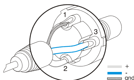
Figure 5: XLR balanced
