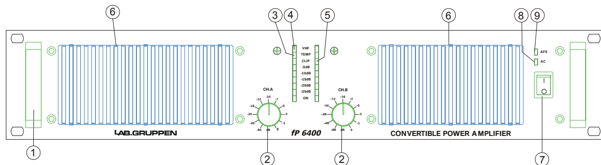
Figure 1: Front panel
