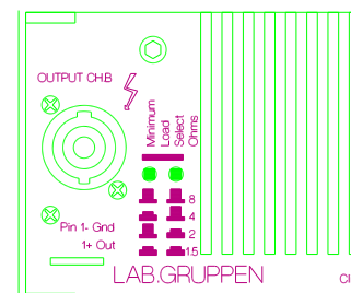
Figure 10. MLS switches on rear panel
