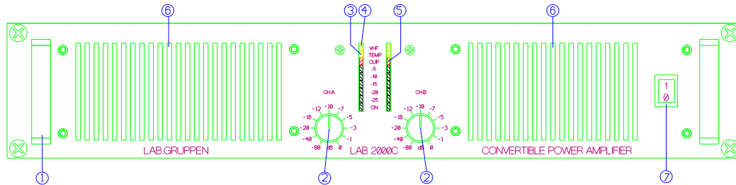
Figure 1. Front panel
