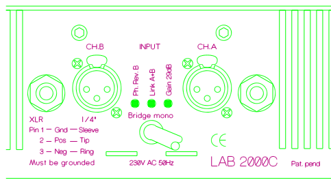
Figure 5. Rear panel connectors
