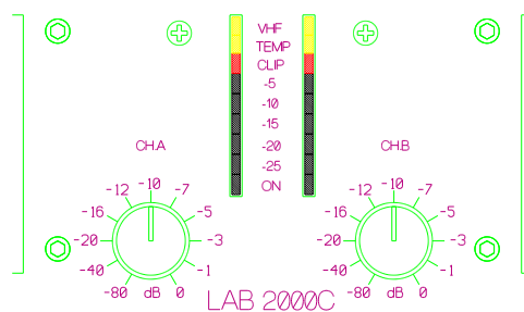
Figure 13. Front indicators
