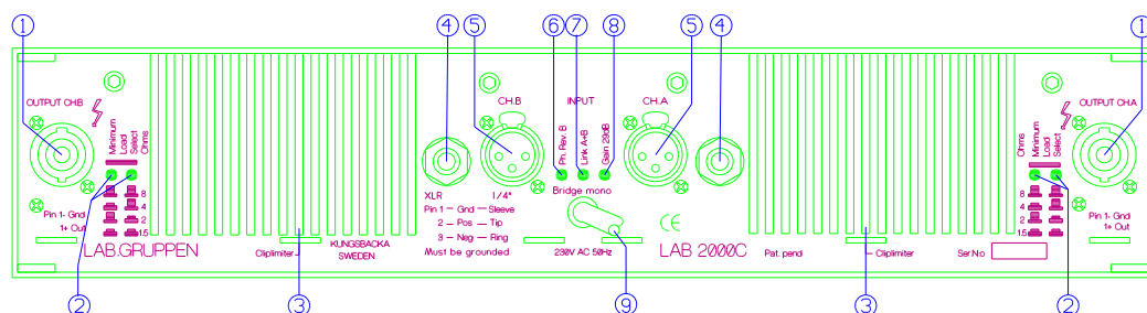
Figure 2. Rear panel
